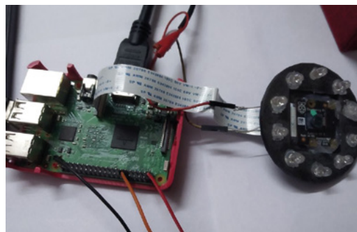
The project's Raspberry Pi NoIR Camera Module is surrounded by a ring of infrared LEDs
