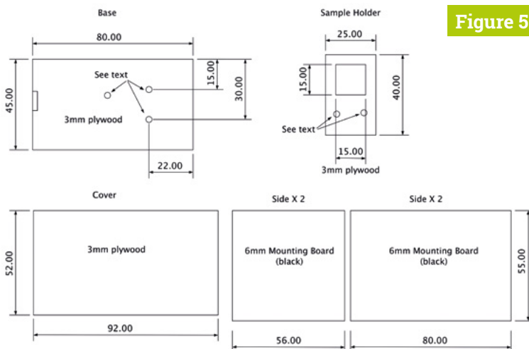
Figure 5 Parts for the Photon Lab's box
