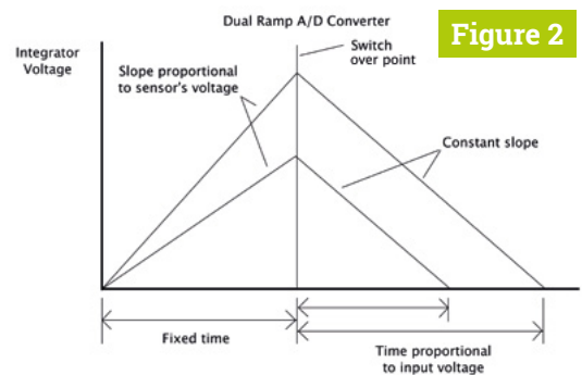
▲ Figure 2 The dual ramp converter in the light sensor chip
