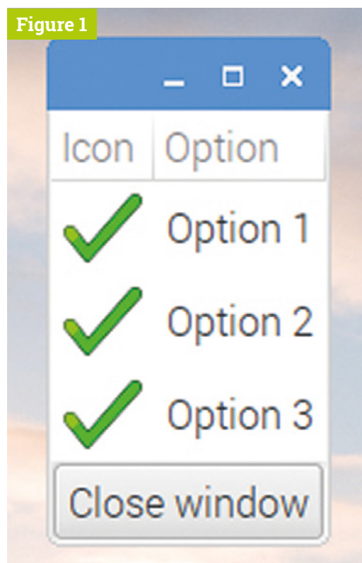
◀ Figure 1 A GtkTreeView with two columns – a pixbuf and some text
