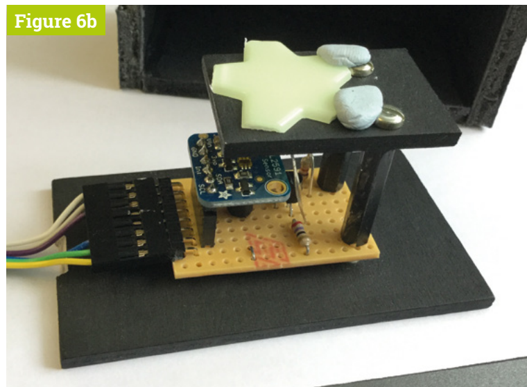
▼ Figure 6b The assembly of the Photon Lab
