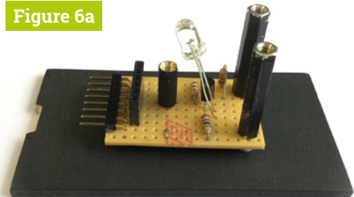
Figure 6a Paint all the parts you can matt black
